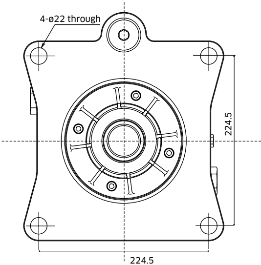
SAE Type
