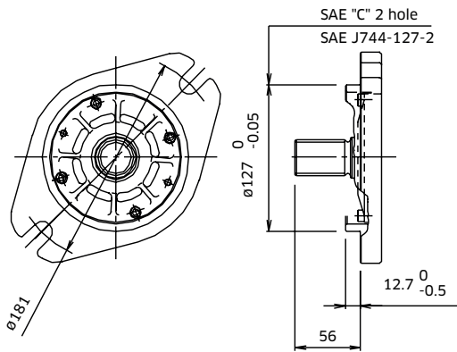
SAE Type
